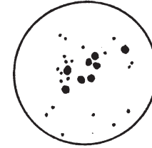
2. Orion Nebula
